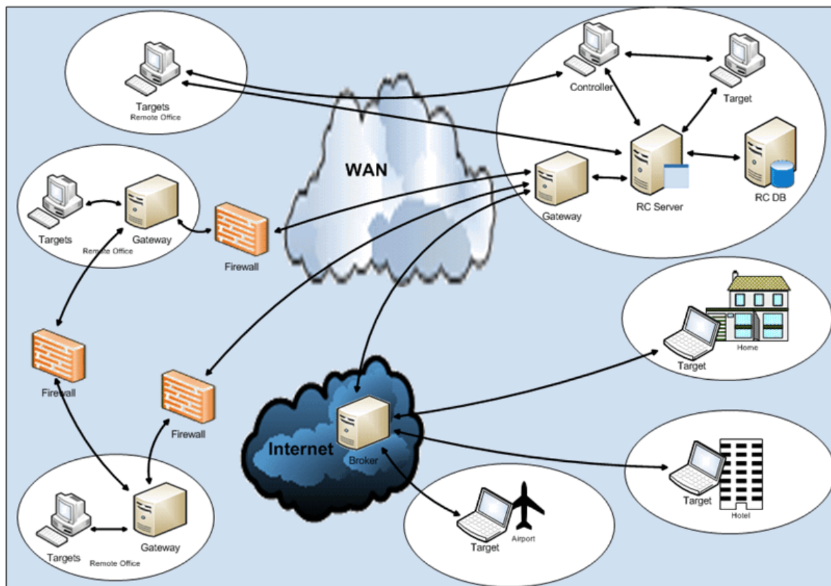
Figure 19: BigFix Remote Control Infrastructure
