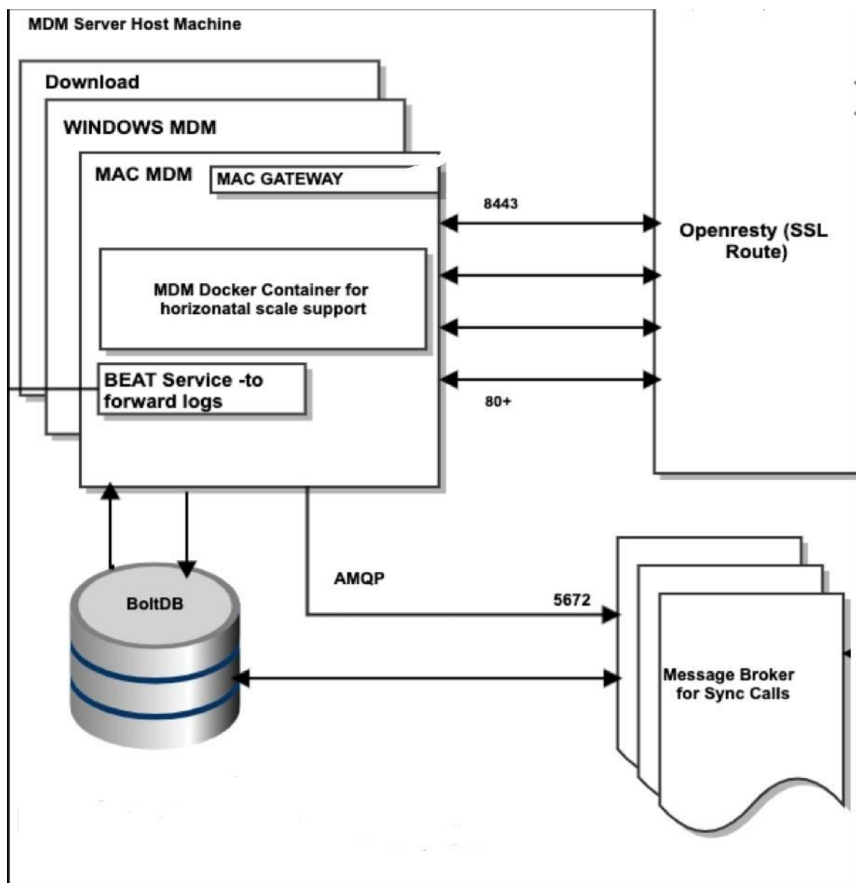
Figure 17: MDM Server Docker Host
